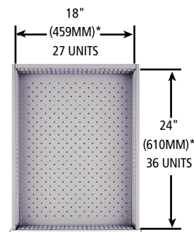
*INSIDE DIMENSIONS
