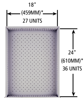
*INSIDE DIMENSIONS
